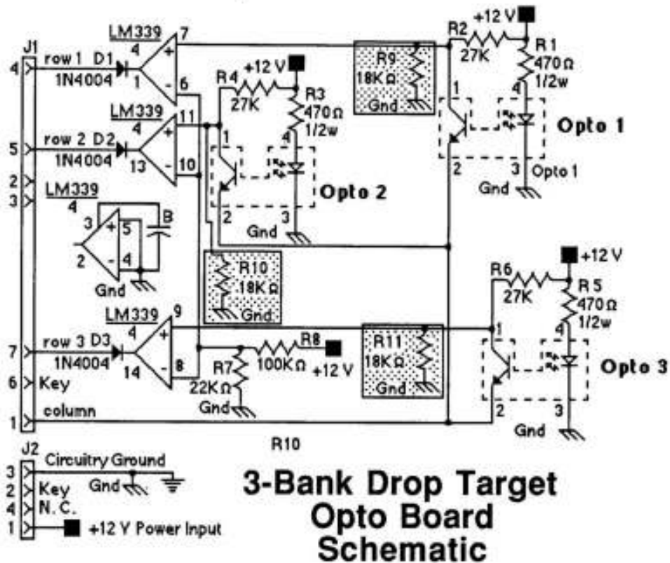
3-Bank Drop Target Opto Board p/n C-12559
