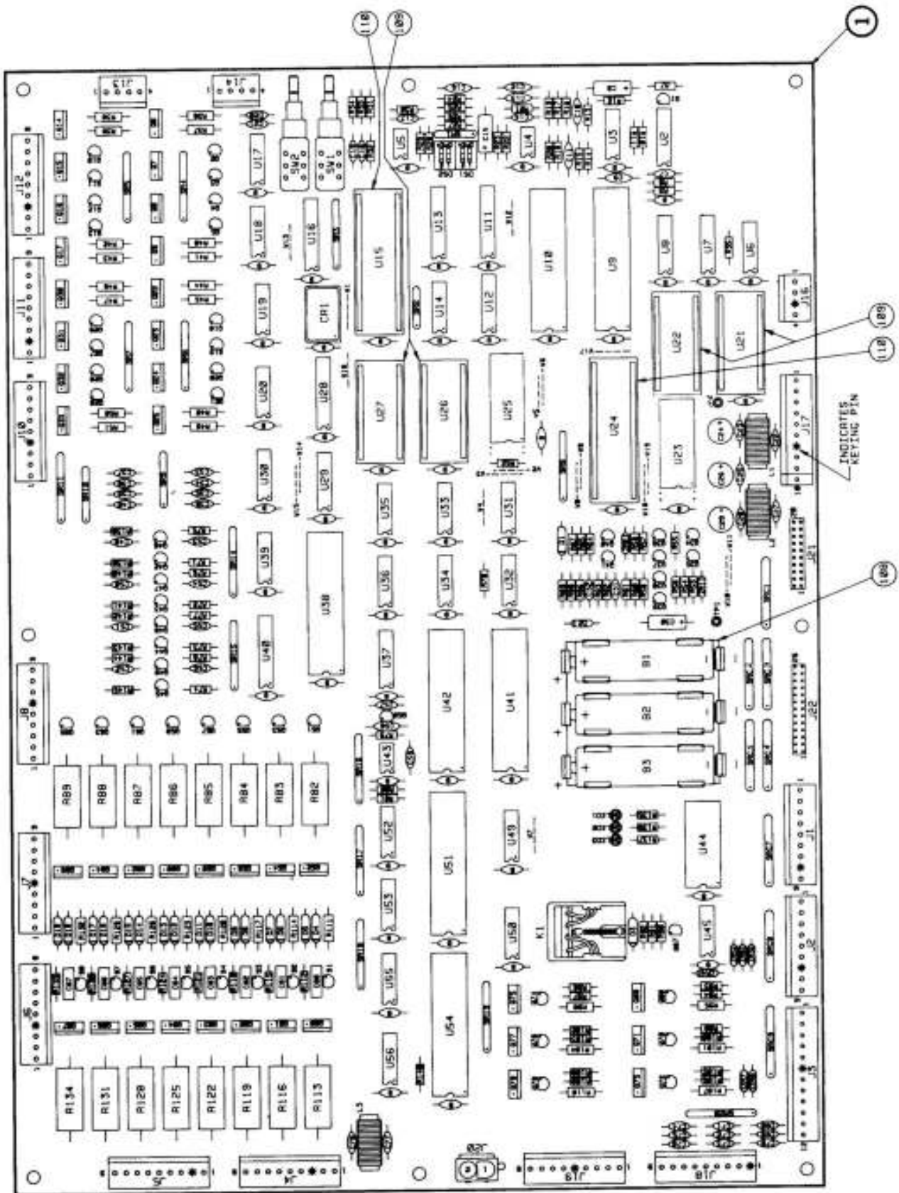
SYSTEM 11B CPU BOARD (D-11883)
