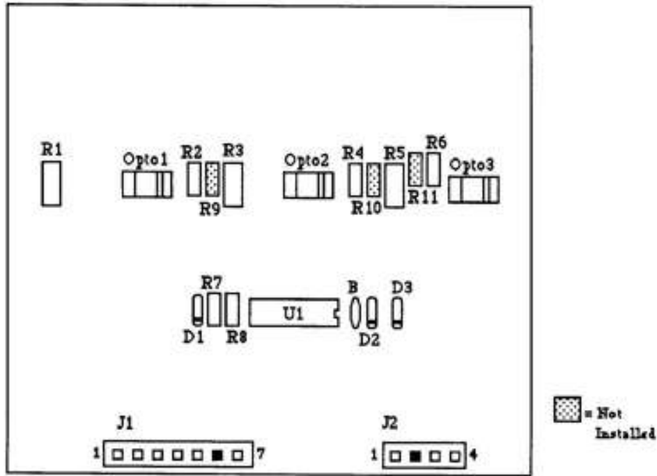
3-Bank Drop Target Opto Board p/n C-12559
