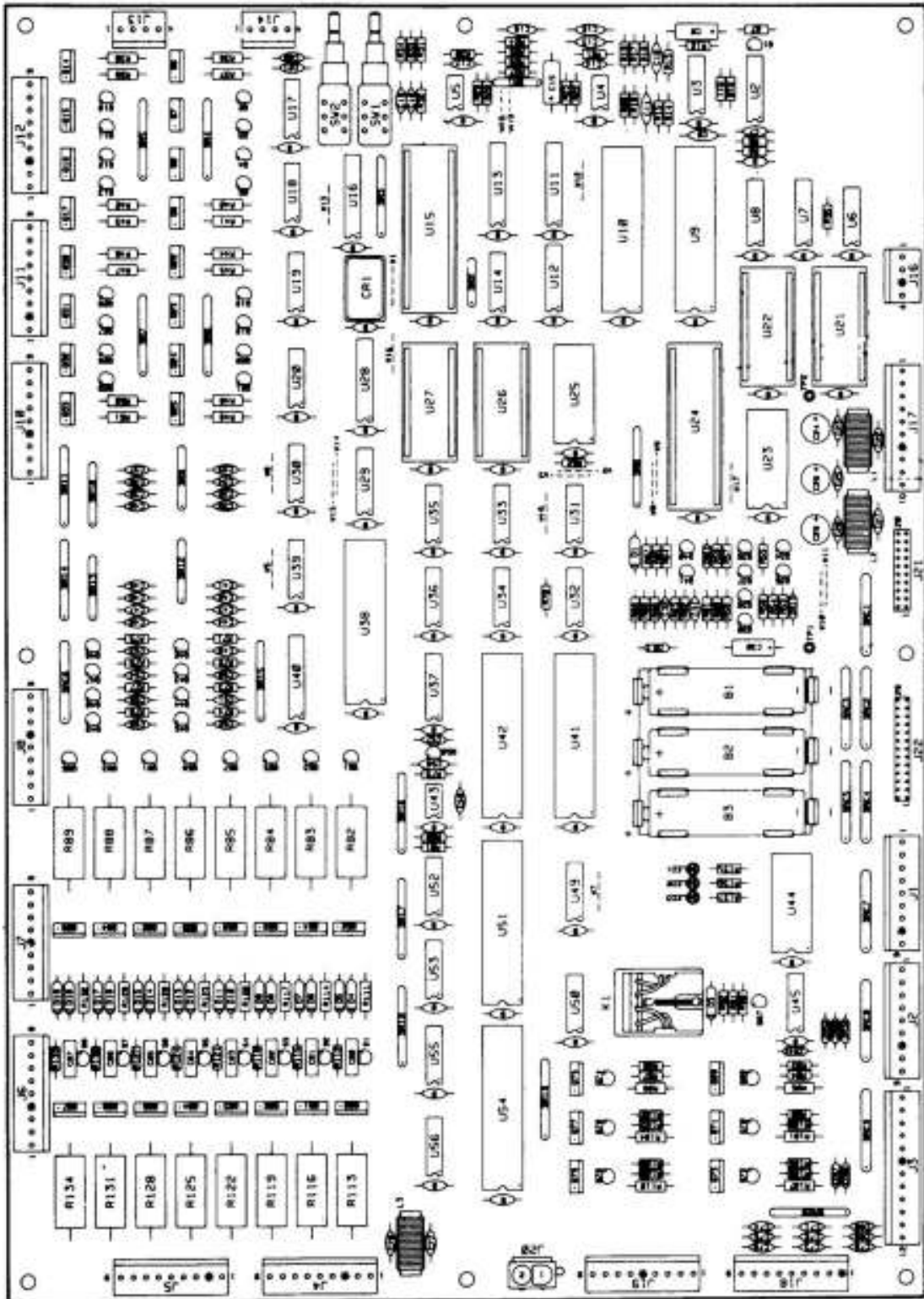
SYSTEM 11B CPU BOARD p/n D-11883
