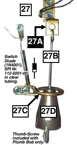
Enlarged Inside Cabinet View of Item 27 (27A, 27B, 27C & 27D), Plumb Bob Tilt Switch.
