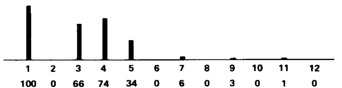
W8 Partials 3, 4, 5, 7, 8, 11,... (no 2, 6, 8, 10,...)
