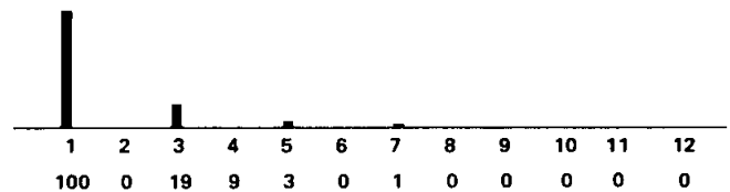
W2 Odd partials somewhat like a square wave
