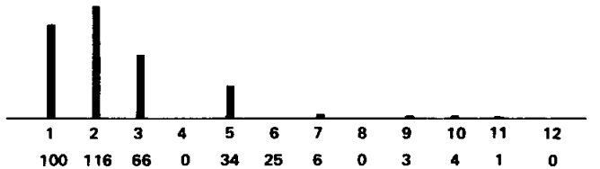
W6 Partials 2, 3, 5, 6, 7, 9, 10, 11,... (no 4,8,...) Second partial is stronger than fundamental.
