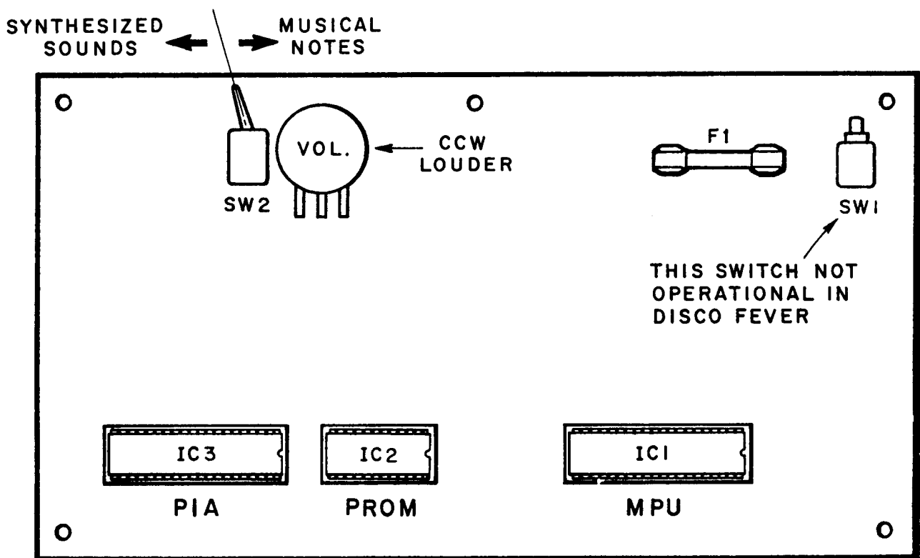
Figure 3. Location of Key Components on Sound Board
