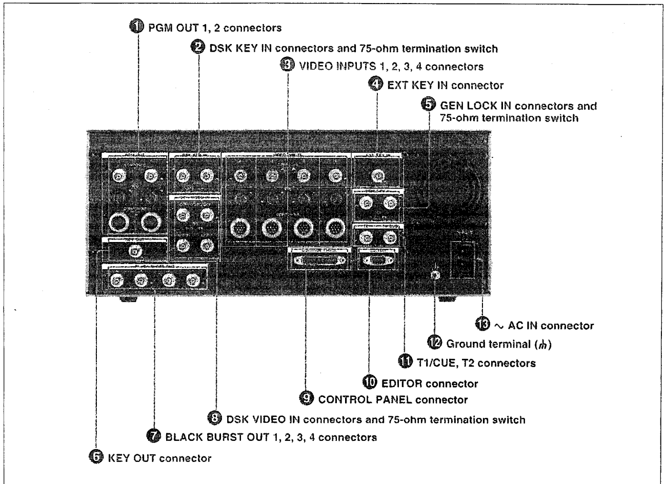
Rear panel
