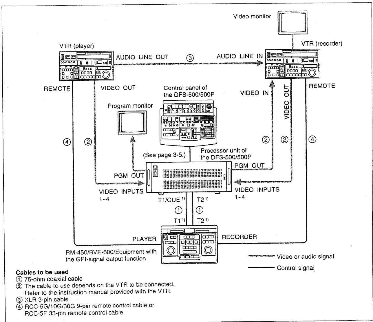
A-roll editing connections
