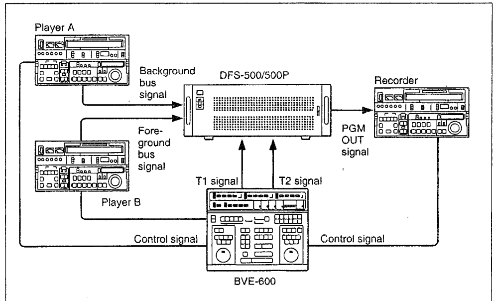
Signal flow
