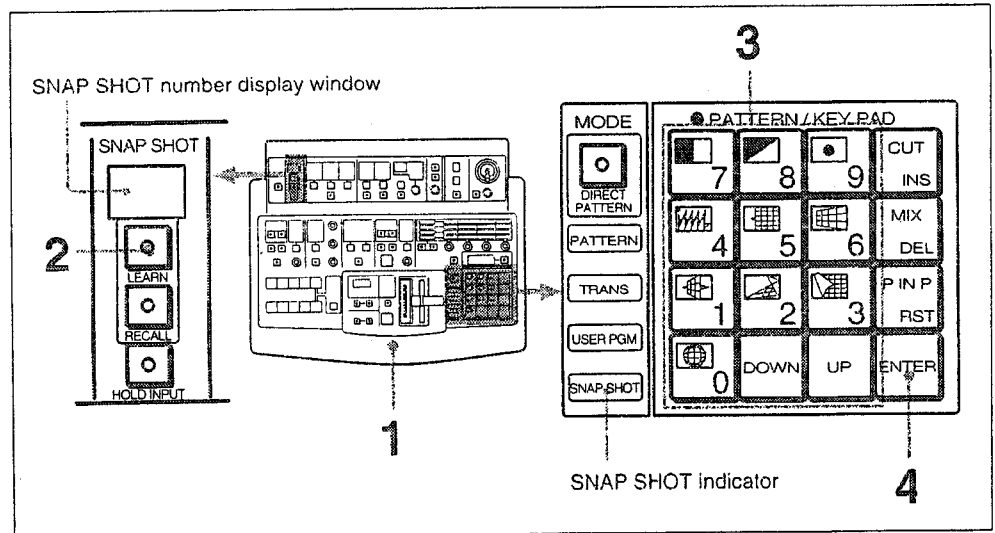
Storing the snap shot data
