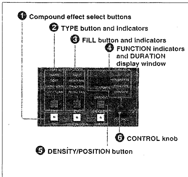
TRAIL/SHADOW section
