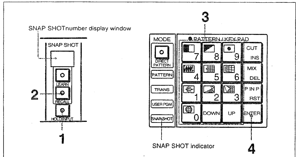
Recalling a snap shot
