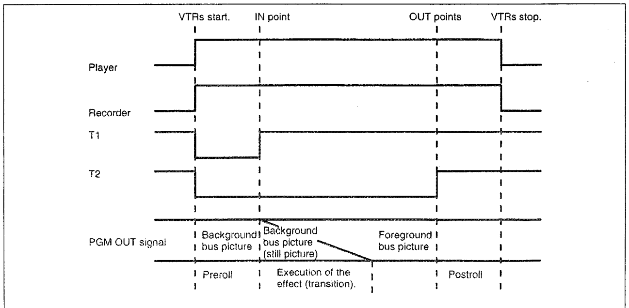
Timing of a trigger signal
