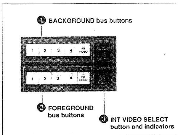
Primary crosspoint bus section
