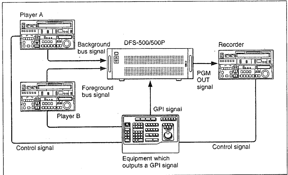
Signal flow
