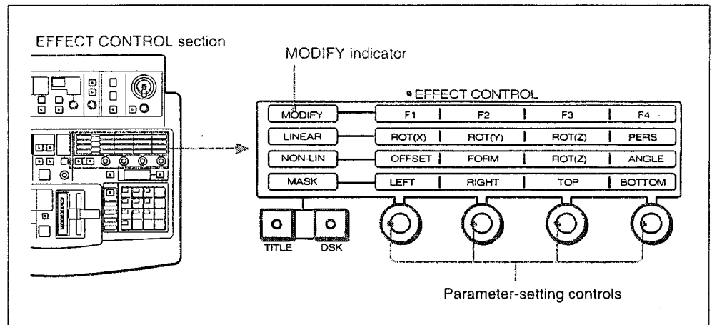
Parameter-setting controls
