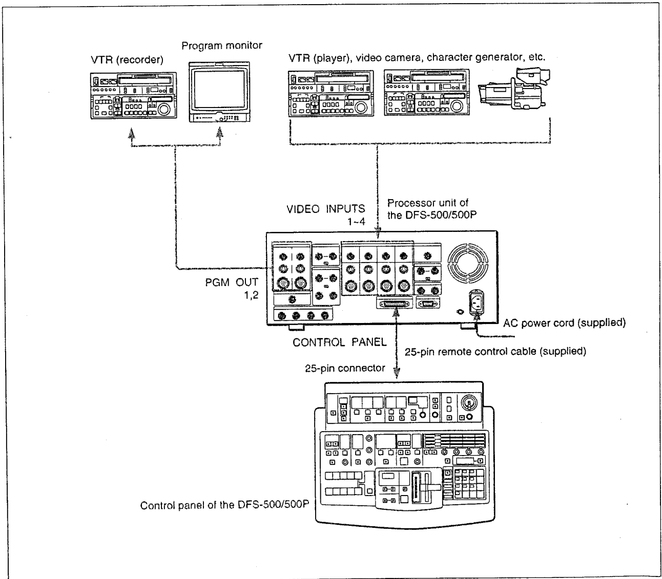
Basic system connections
