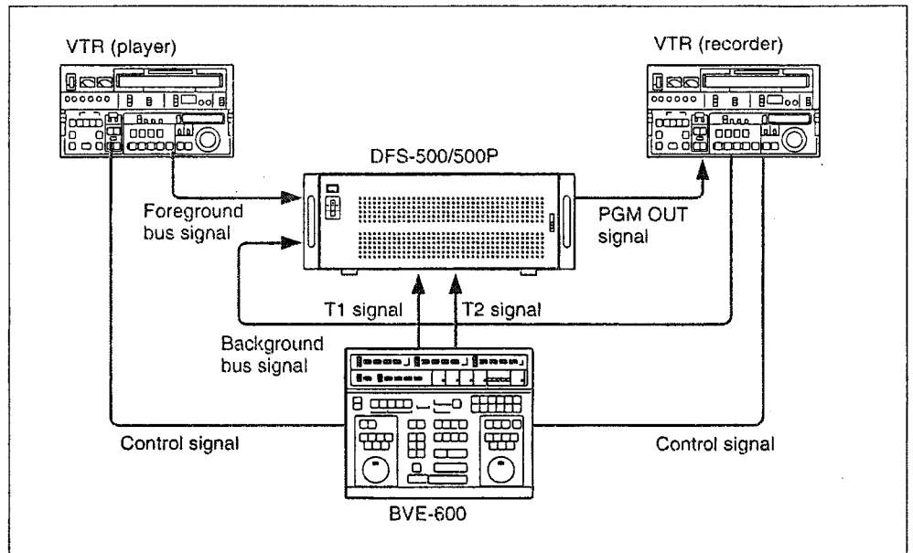
Signal flow
