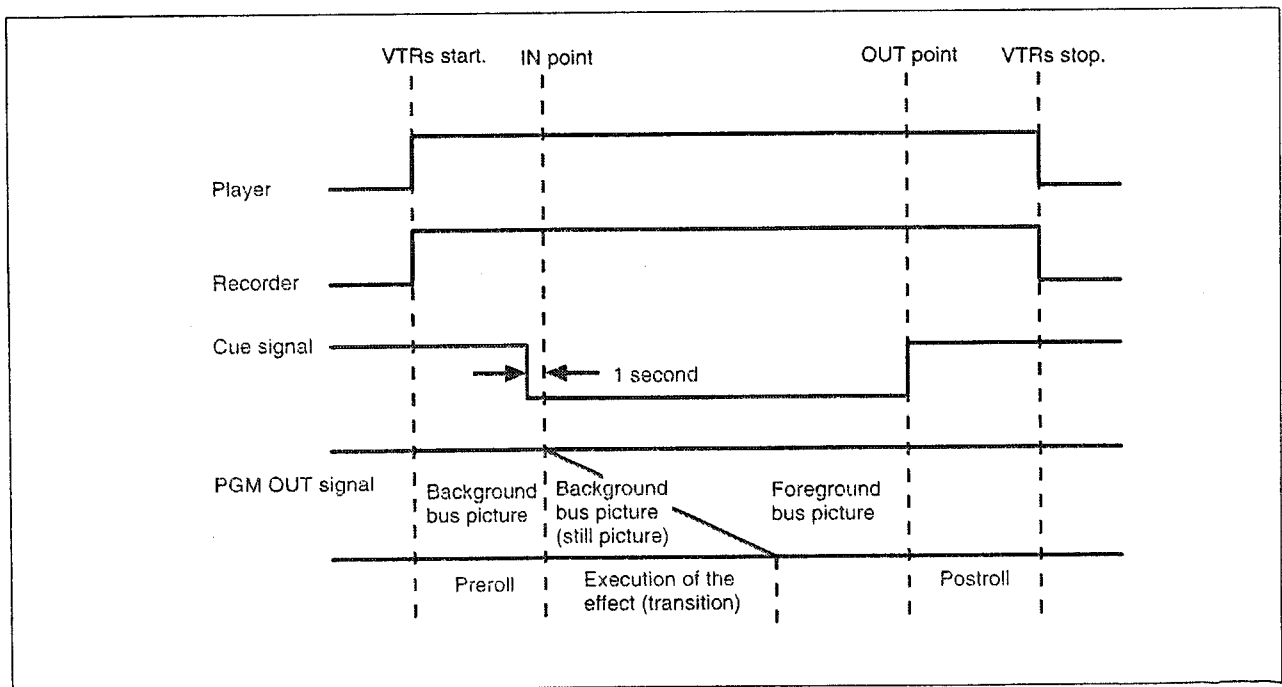
Timing of a cue signal
