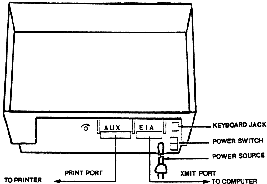
Figure 3-5 Detail Of Cabinet Illustrating Comm Ports
