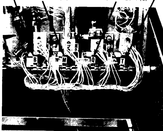
BALL SAVE RELAY (B) MOTOR RELAY (M) TILT RELAY (T) GAME OVER RELAY (Q)
