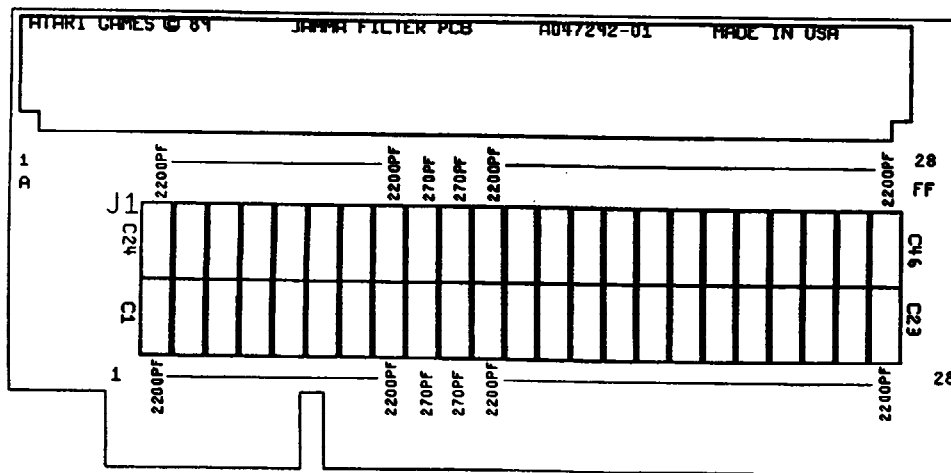
Figure 4-7 JAMMA Filter PCB Assembly A047292-01 A
