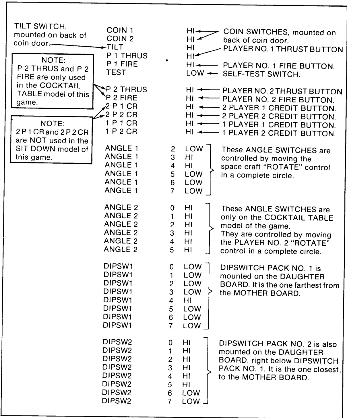
FIGURE 13 DISPLAY EXPLANATION
