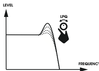
FIGURE 4. How LPQ affects the audio signal.
