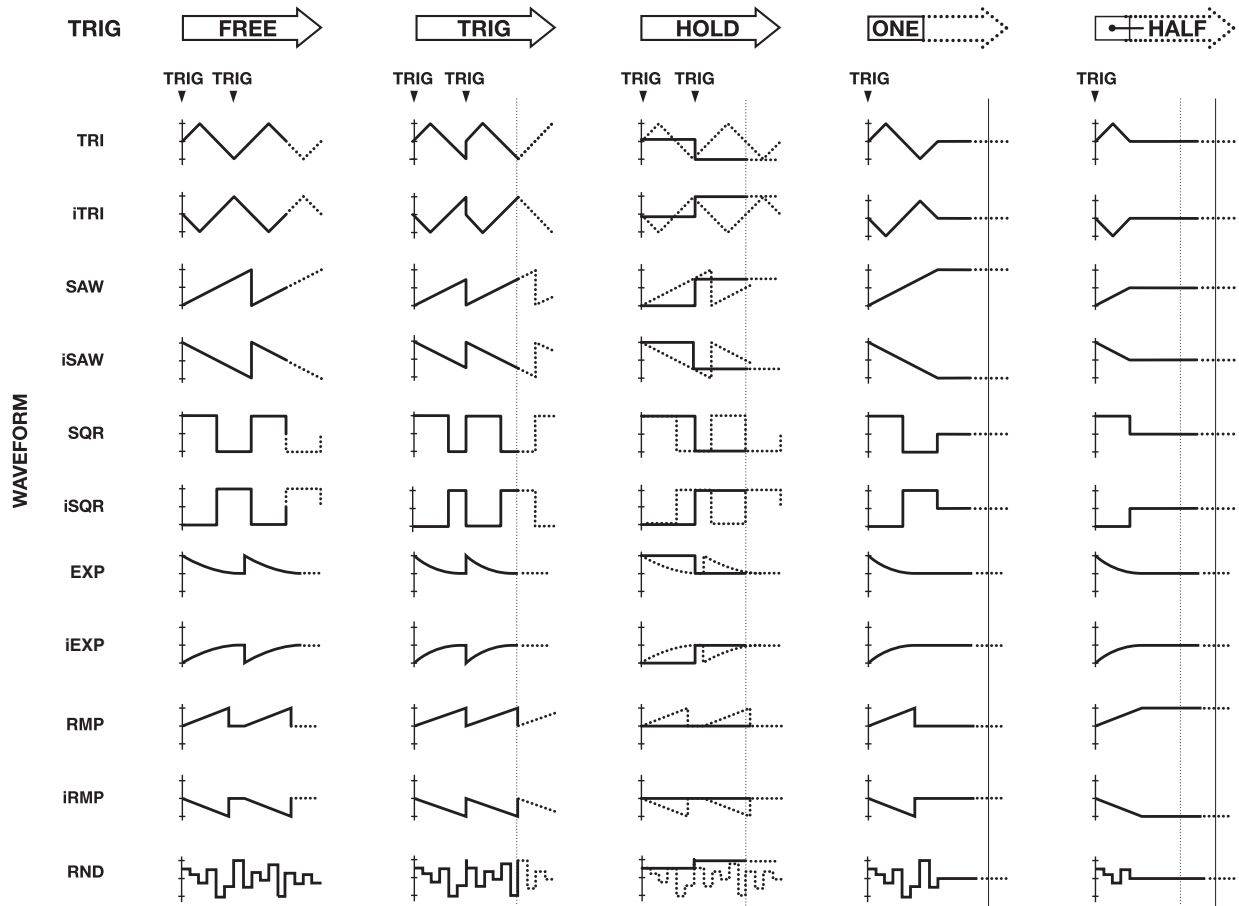
FIGURE 6. Monomachine LFO waveform and trig modes
