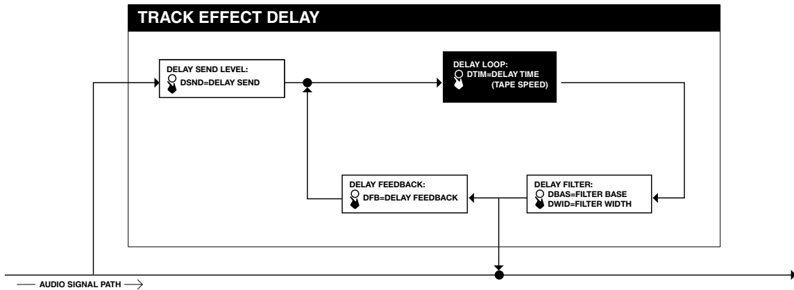
FIGURE 5. The function of the delay
