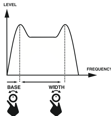
FIGURE 3. How the BASE and WDTH parameters works.
