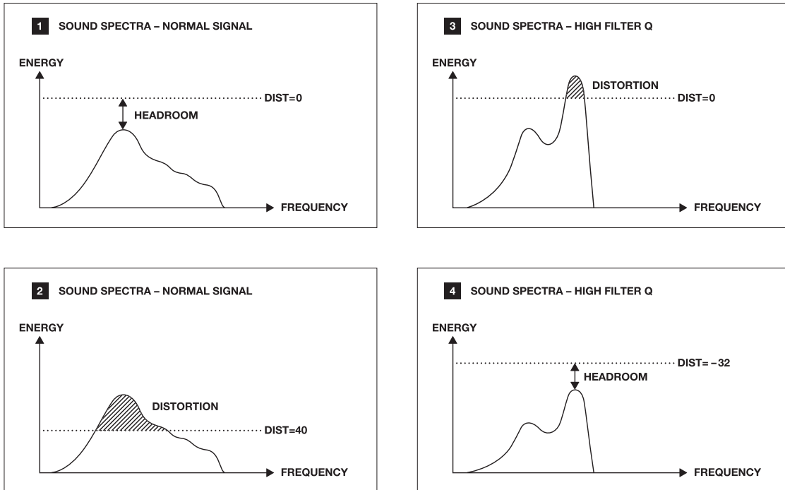
FIGURE 2. Simplified visualisation of headroom and distortion
