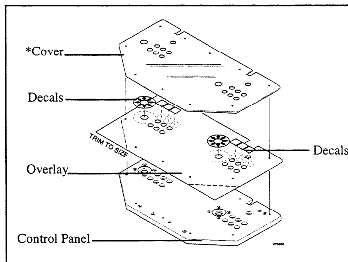
Figure 1 Overlay Installation
