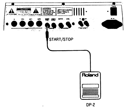
Rear Panel
