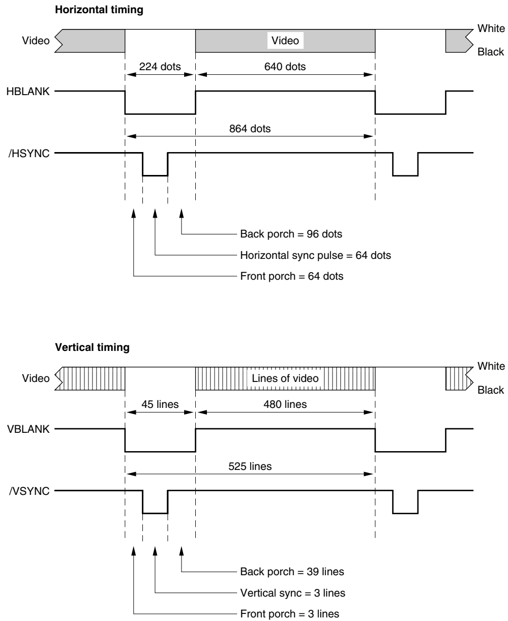
Figure 2-3 Standard video timing
