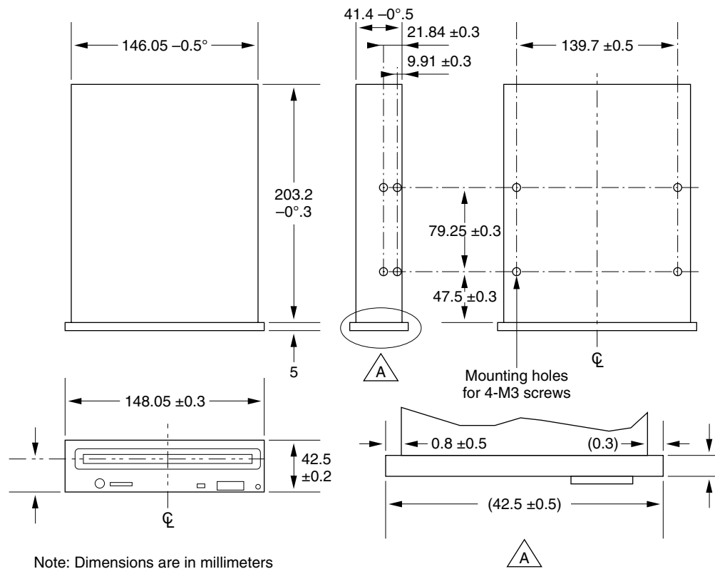
Figure 5-5 Dimensions of the CD-ROM drive
