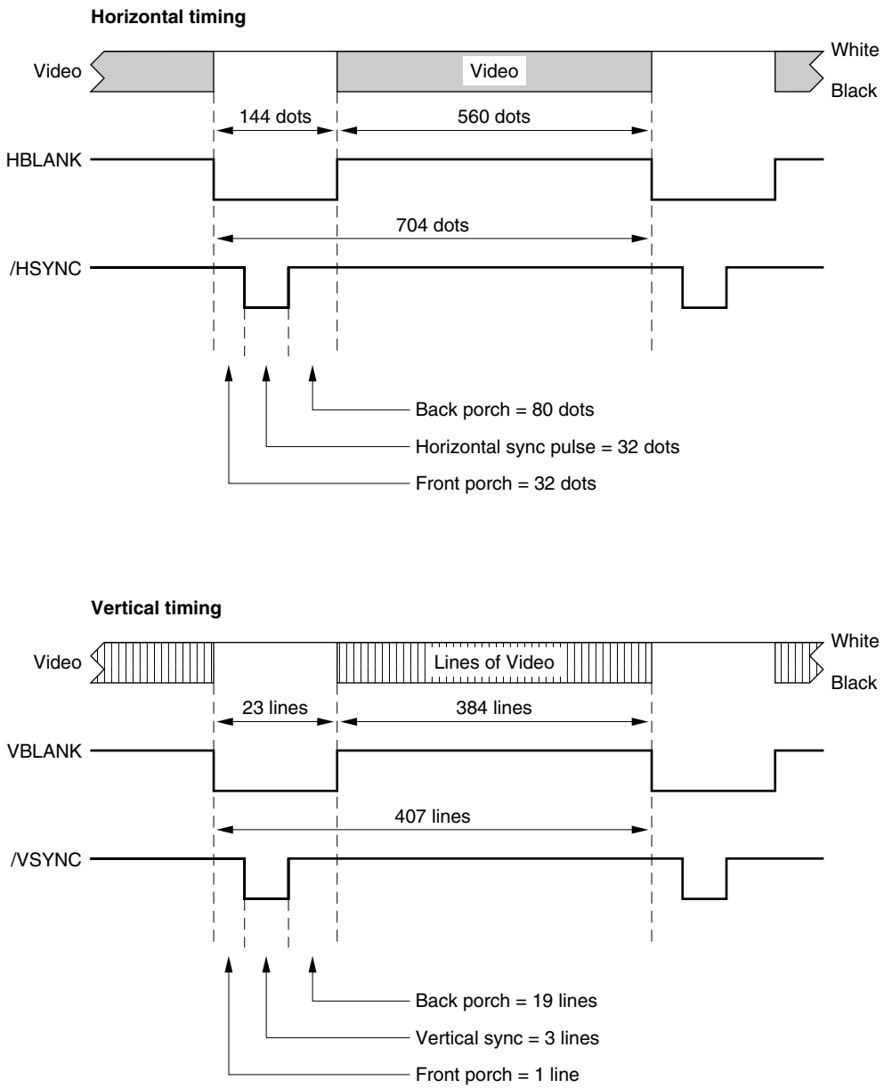
Figure 2-4 Video timing for the Apple IIe card
