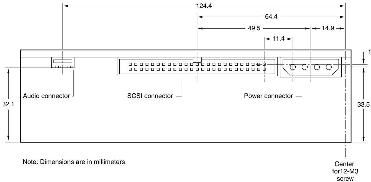
Figure 5-3 Connector locations on the CD-ROM drive
