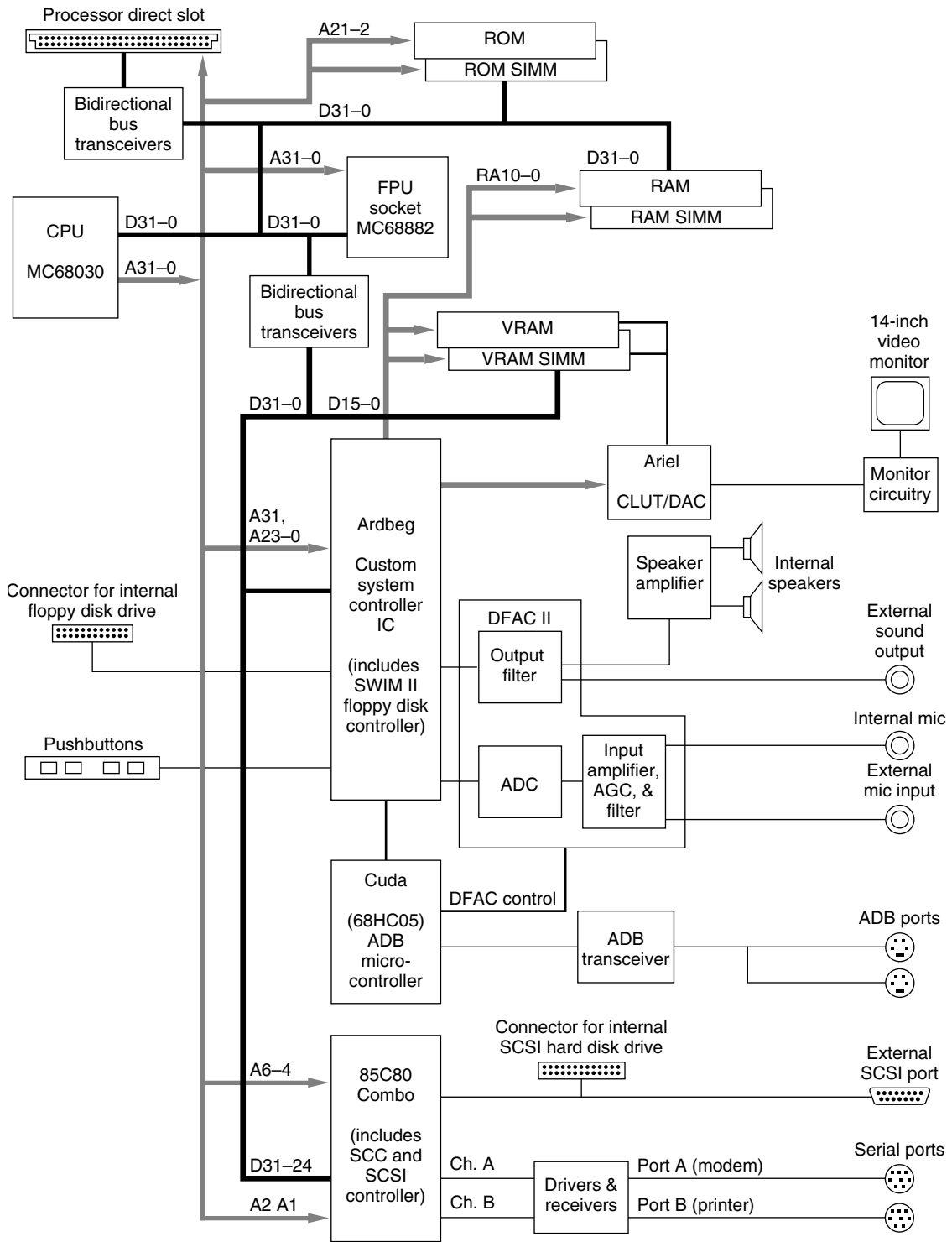
Figure 2-1 Block diagram
