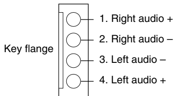
Figure 5-7 Pins on the CD-ROM audio connector
