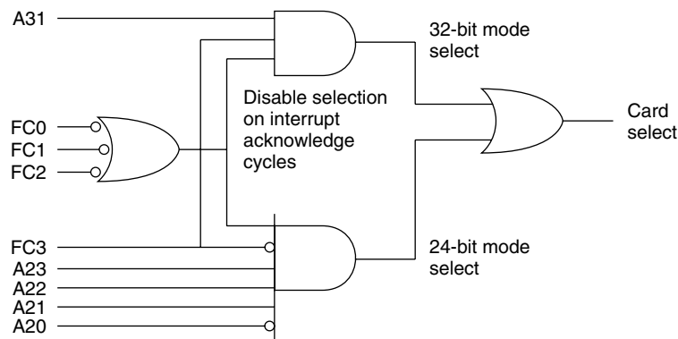
Figure 3-1 Generating the card select signal
