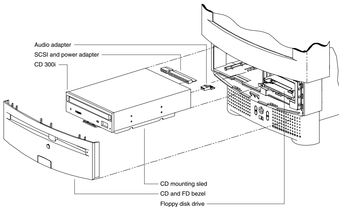
Figure 5-1 Installation of the internal CD-ROM drive
