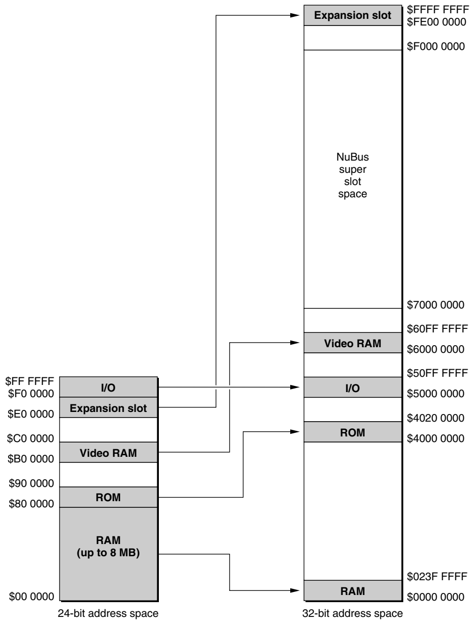
Figure 2-2 24-bit and 32-bit address maps
