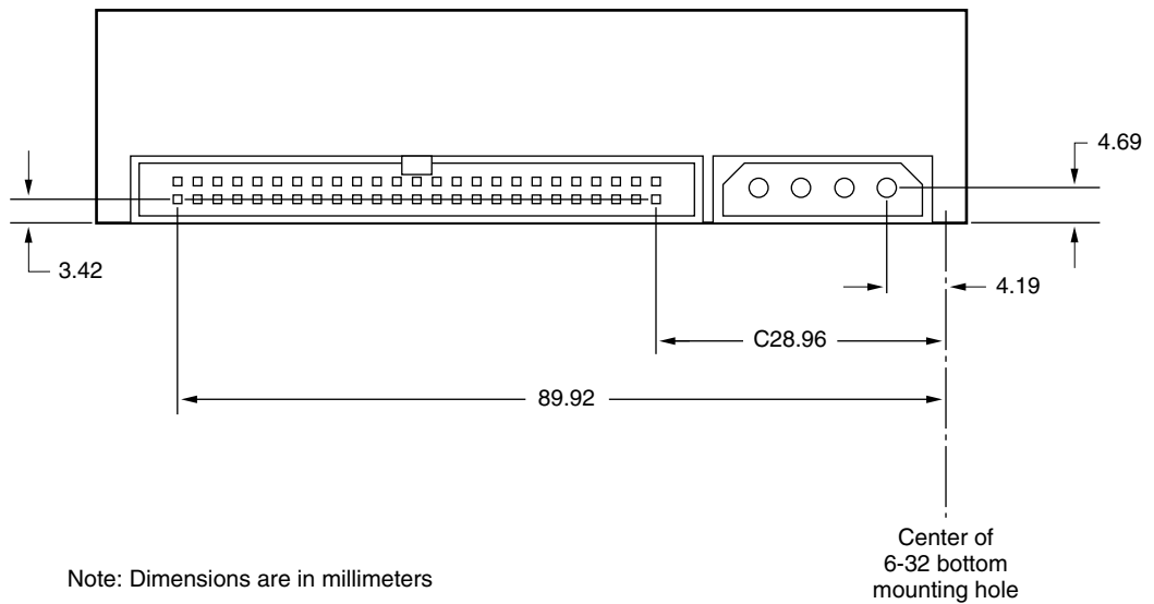
Figure 5-5 Dimensions of the CD-ROM drive
