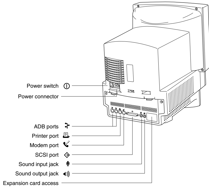
Figure 1-2 Back view of the Macintosh LC 520 computer
