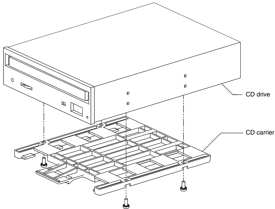
Figure 5-6 The AppleCD 300i mounted on the sled
