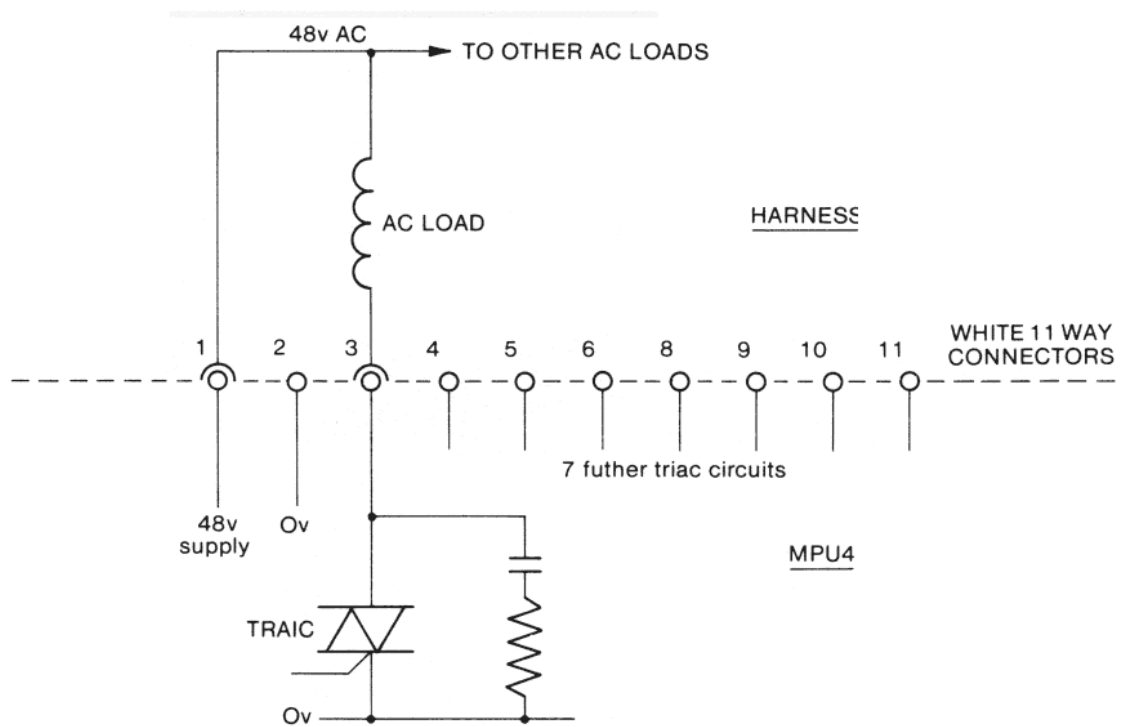
FIGURE 19 TRIAC CIRCUITS
