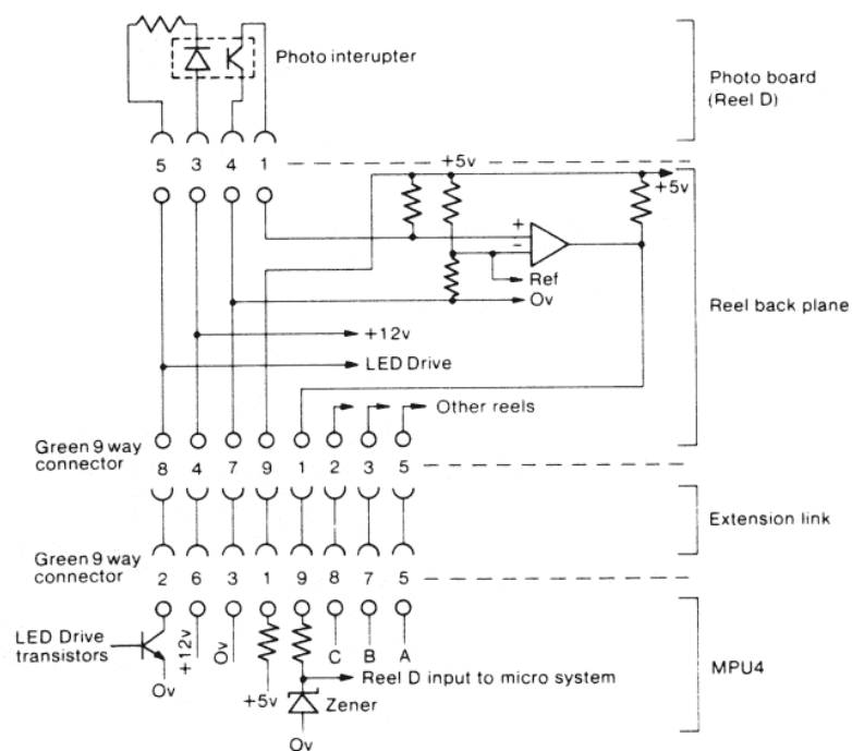
FIGURE 22 REEL PHOTO CIRCUIT (Shown for reel D)
