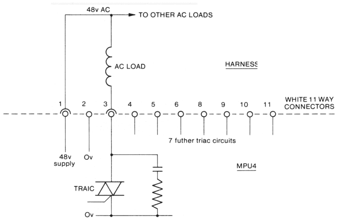
FIGURE 19 TRIAC CIRCUITS
