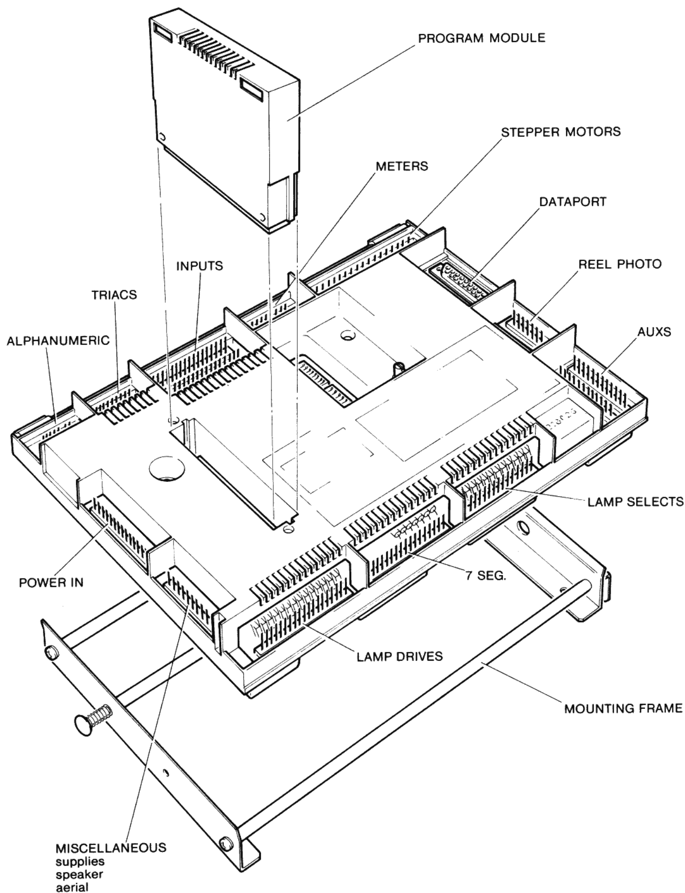
FIGURE 10 MPU 4
