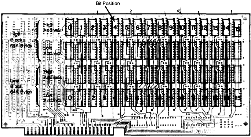
A26 Assembly
