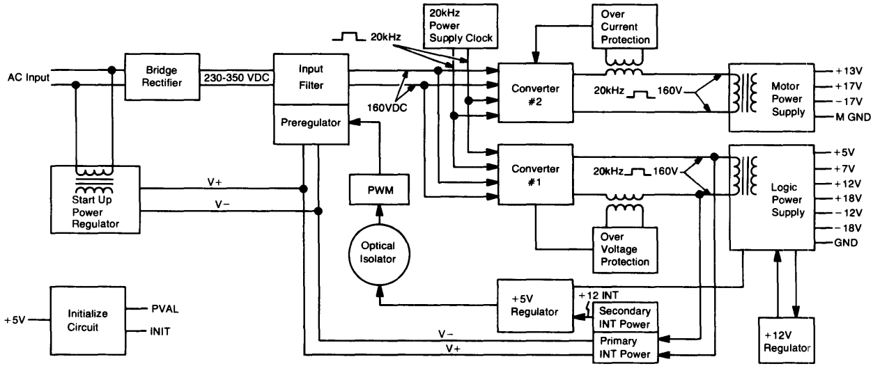
Opt. 1XX Power Supply Block Diagram, A80
