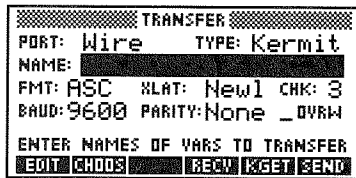
The Wire TRANSFER Screen
