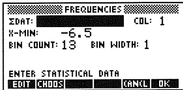
The FREQUENCIES Screen
