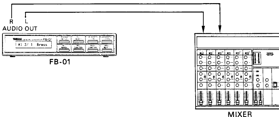
Figure 2: Connecting the FB-01 to a Stereo Mixer or Amplifier
