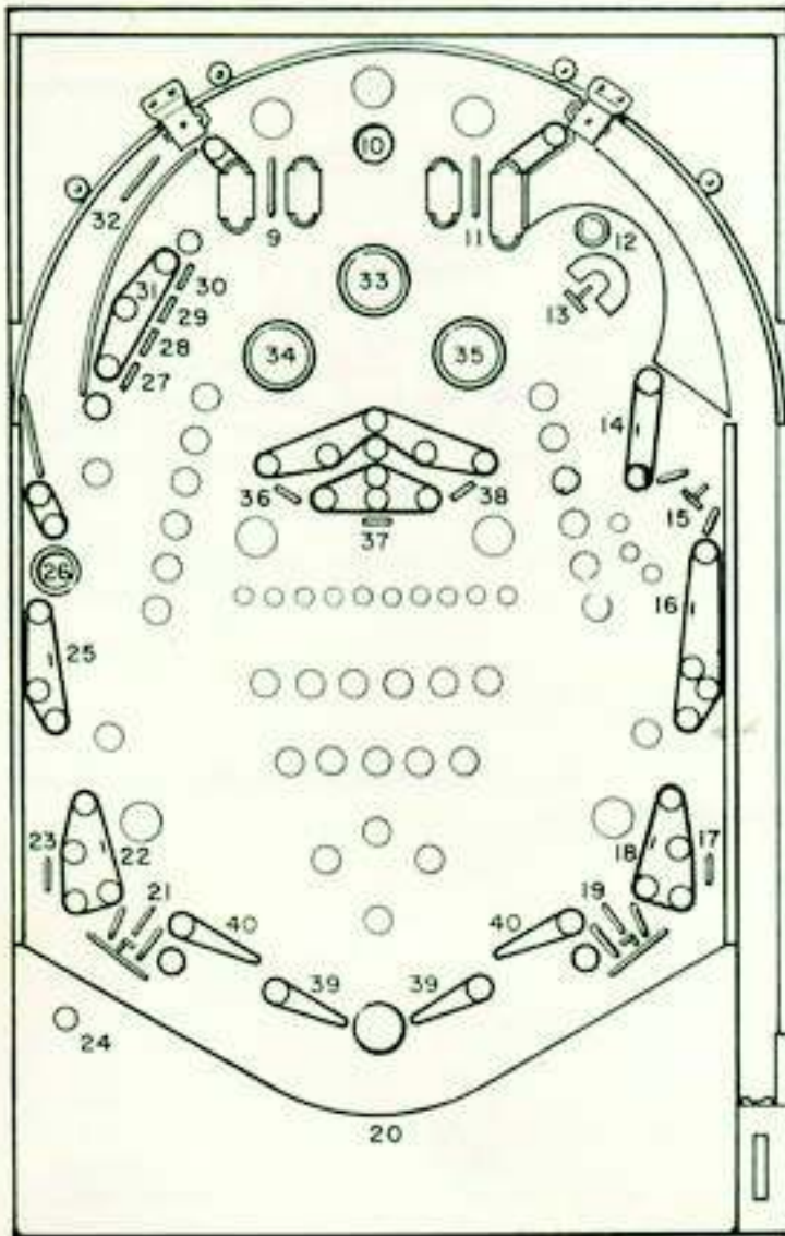
Figure 7. Location of Playfield Switches
