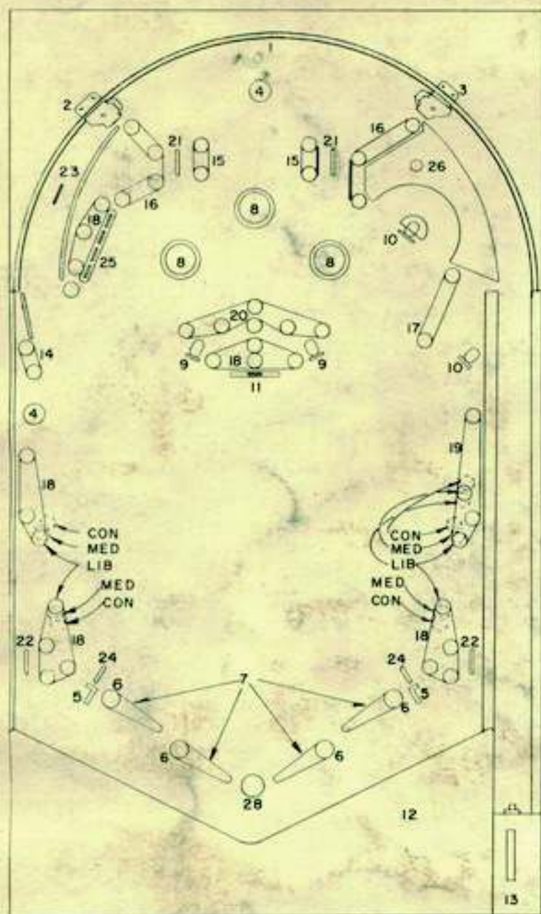
Figure 12. CONTACT Spare Parts Identification and Post Adjustment Details
