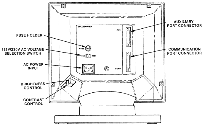
Figure 2-1. Back View of the Display Unit
