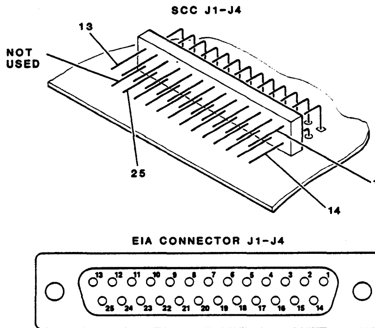
Figure 9: SCC PIN NUMBERING
