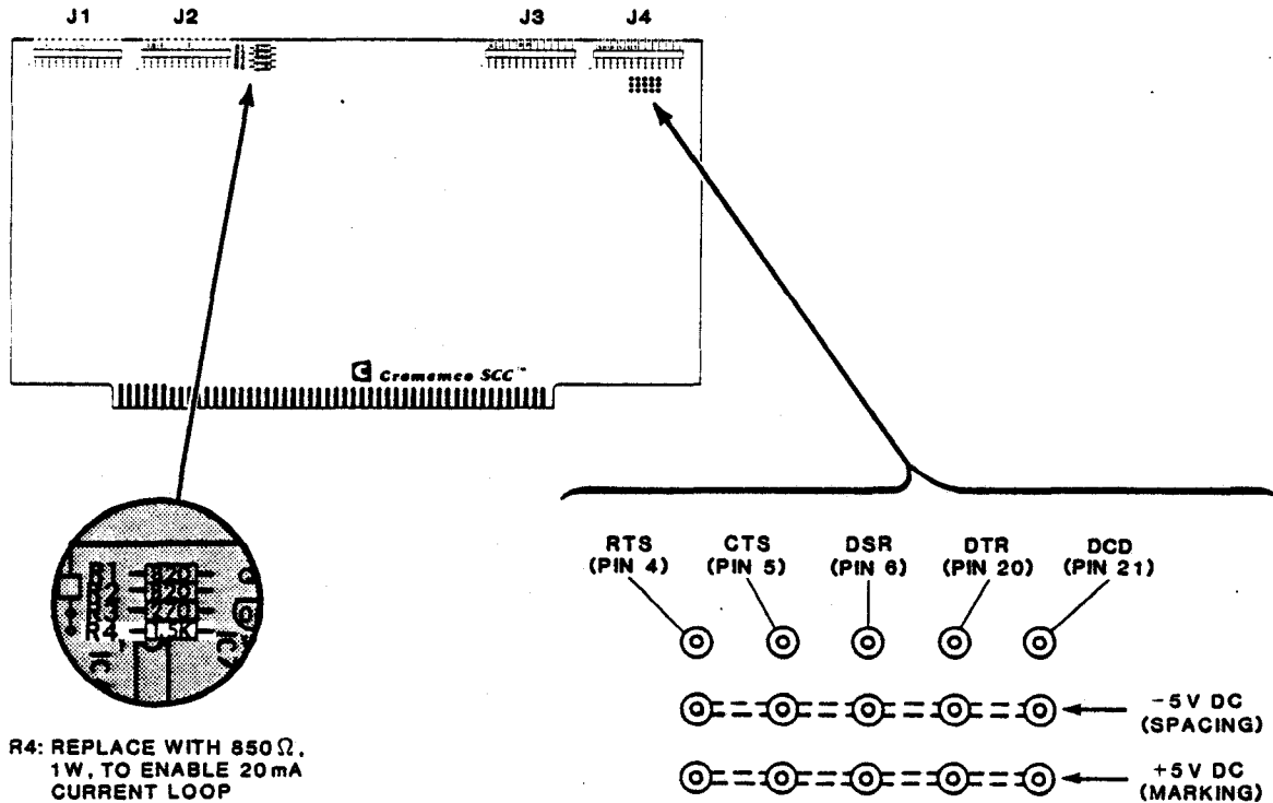
Figure 16: SCC MODEM CONTROL JUMPER PADS
