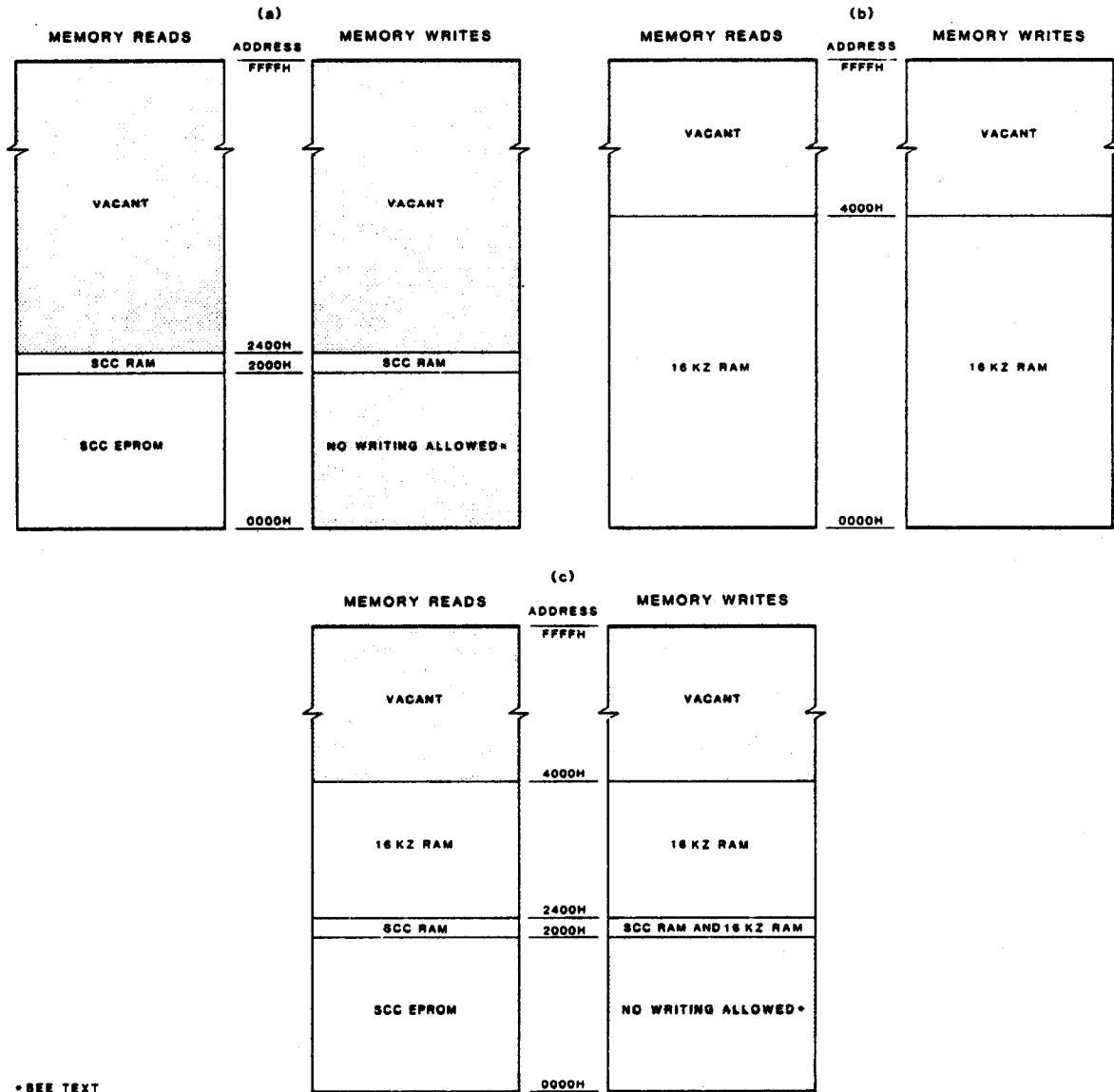
Figure 7: EXAMPLE 2 MEMORY MAPS
